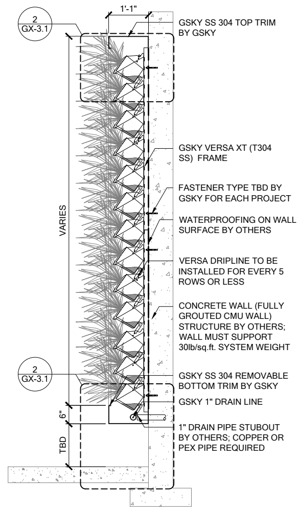
3 SECTION SCALE 3/8" = 1'-0"
