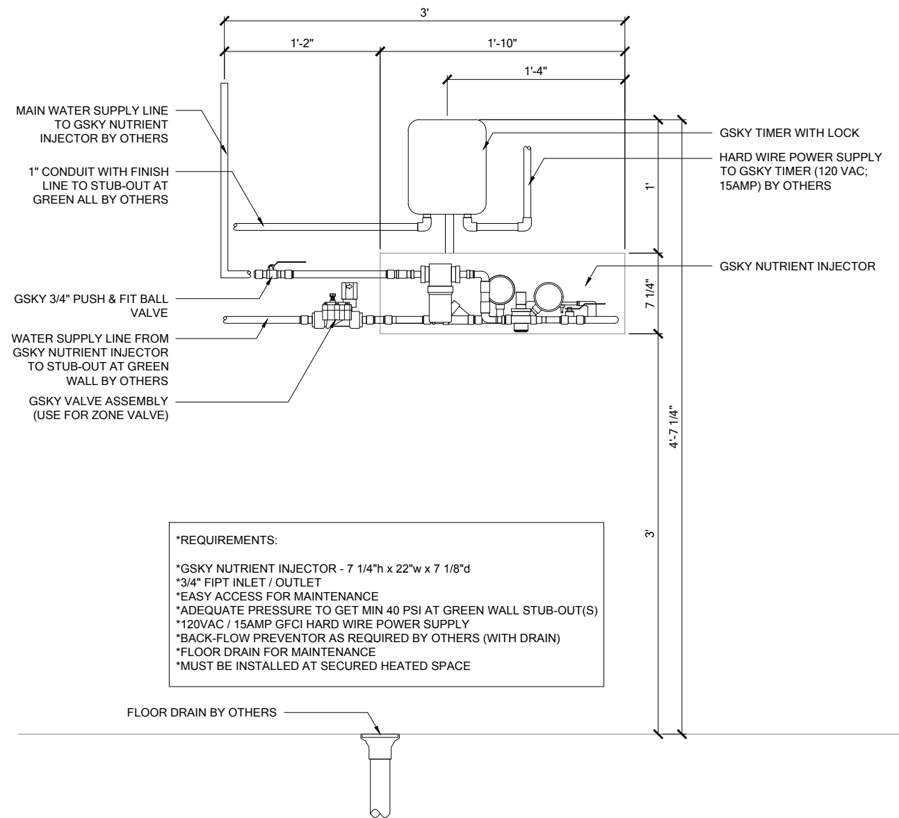
1 SINGLE ZONE - ELEVATION SCALE 1 1/2" = 1'-0"
