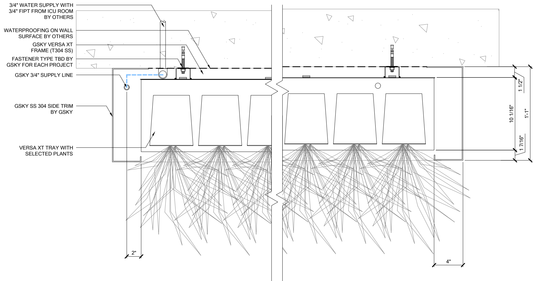
1 PLAN DETAIL SCALE 1 1/2" = 1'-0"
