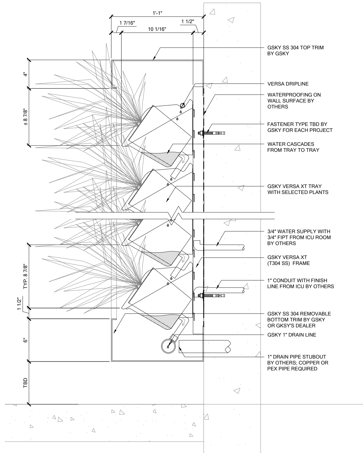
2 SECTION DETAIL SCALE 1 1/2" = 1'-0"
