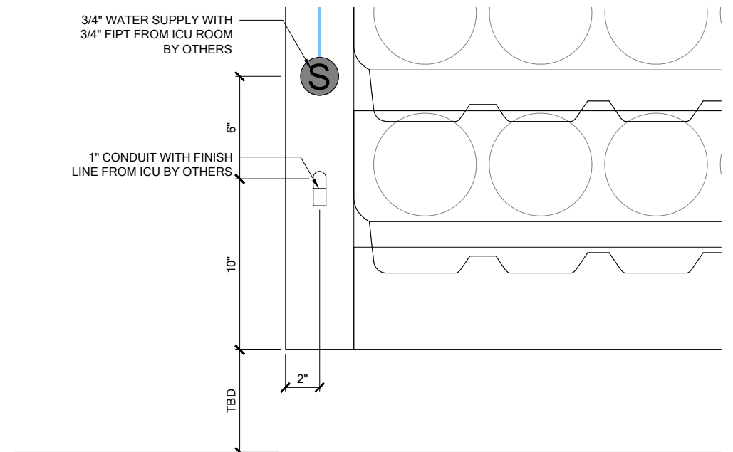
3 ELEVATION DETAIL SCALE 1 1/2" = 1'-0"
