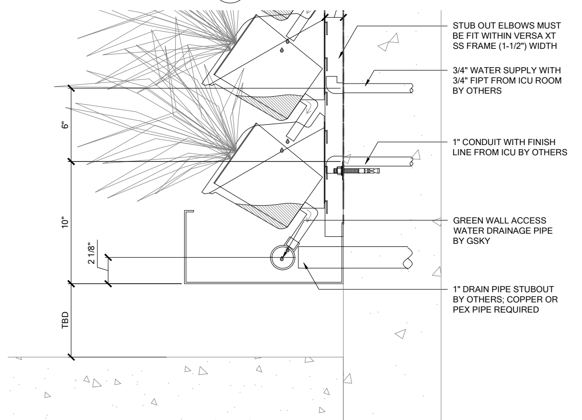
2 SECTION SCALE 1 1/2" = 1'-0"
