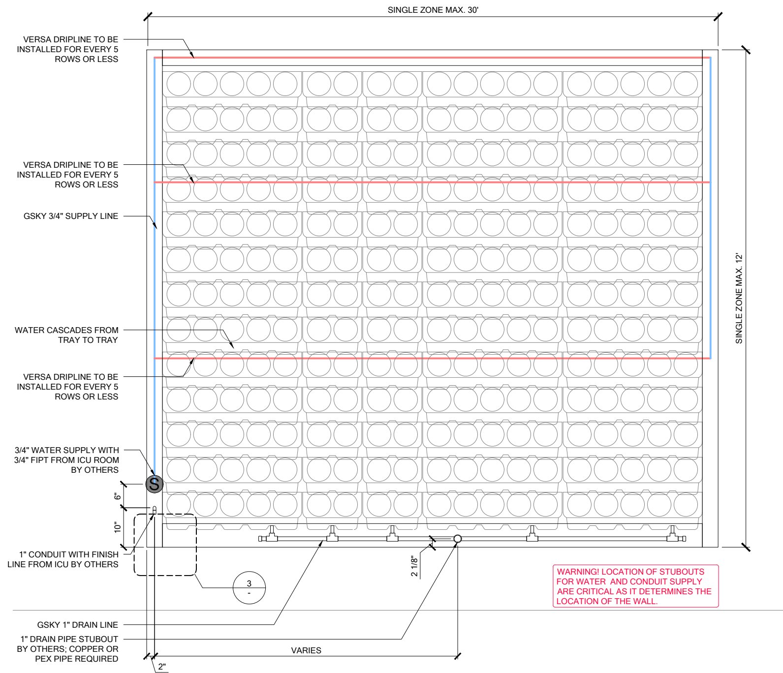
1 ELEVATION SCALE 1/2" = 1'-0"
